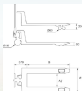
Dimensions: A2 = 240 mm
